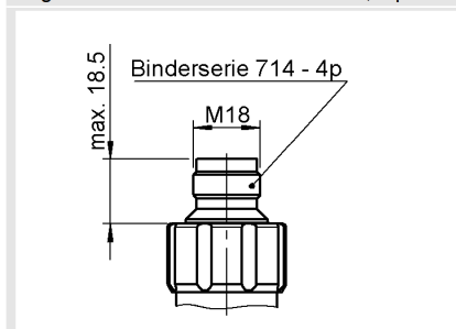
Plug connector Binder series 714 M18, 4 pole
