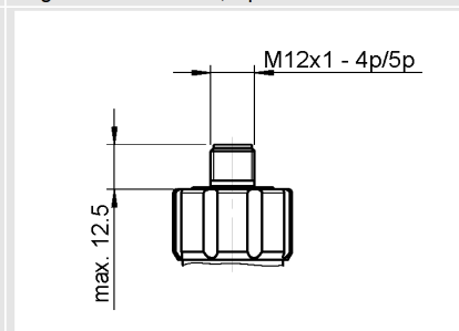
Plug connector M12x1, 4 pole
