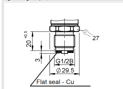
G1/2 B DIN EN 837 / external Tightening torque, recommended: 45 Nm
